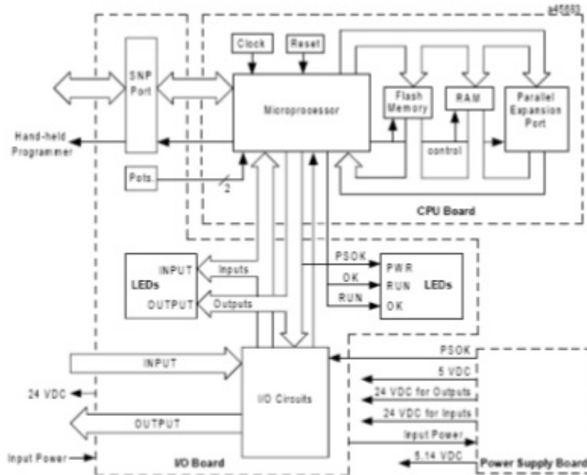
Figure of Micro PLC Functional Block Diagram
